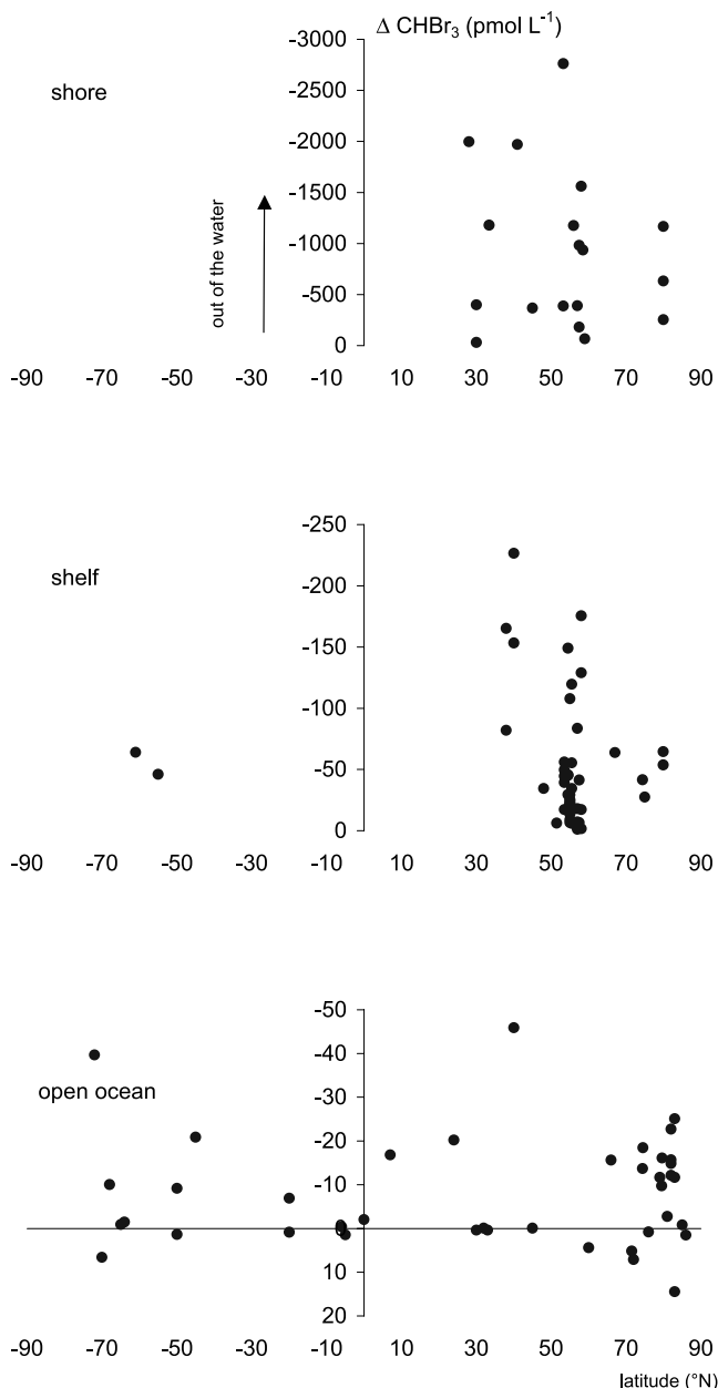
Figure 7. \Delta c \text{ CHBr}_3 [pmol L -1 ], as a function of latitude of oceanic bromoform for near shore, shelf and open ocean regimes ( \Delta c \text{ CHBr}_3 = actual water concentration-concentration in equilibrium with air).
