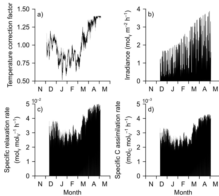
Fig. 9. Temperature correction factor (a), irradiance (b), specific relaxation rate from photosynthetic SU2 (c) and carbon assimilation rate resulting from photo-synthetic SU3 (d) at Pt. Judith Pond during year 2. Black is for the North S. latissima line and the grey is for the South line.
