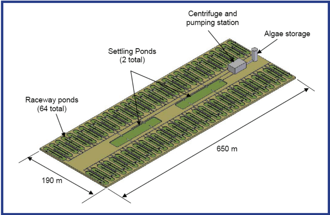
Figure 6: Scaled model of algae farm with raceways and settling ponds (Sazdanoff, 2006)
