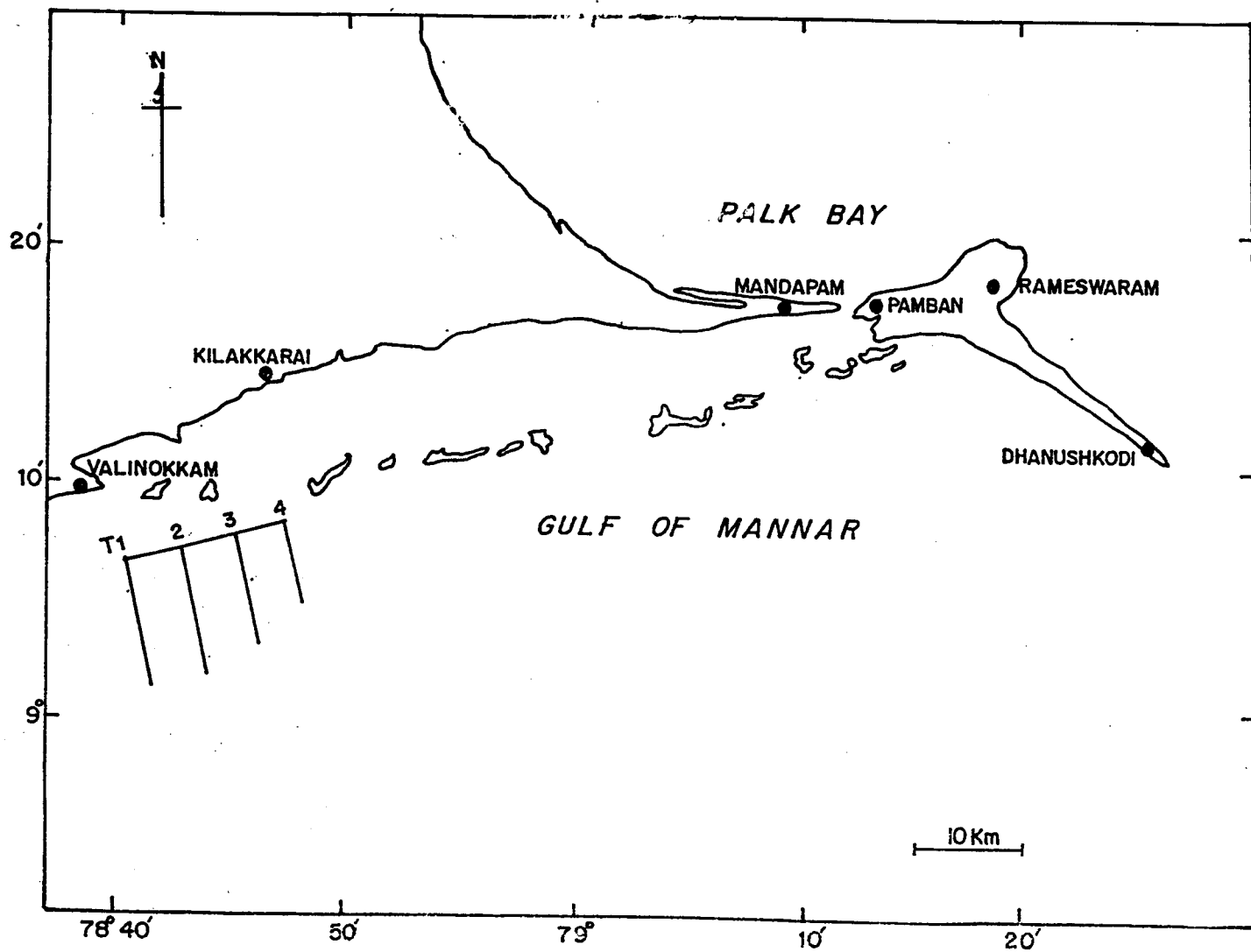
Fig.1 Map showing the location of transects in the area surveyed from Valinokkam to Kilakkarai.
