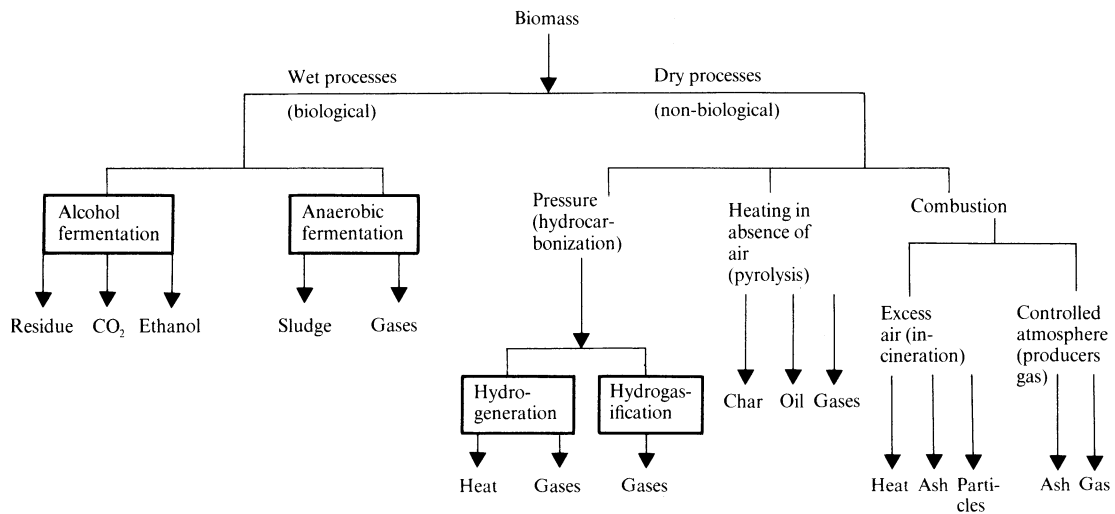
Figure 2. Production of 200° proof anhydrous ethyl alcohol from starch, sugar or cellulosic materials.
